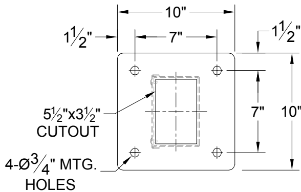
BASEPLATE DETAIL
